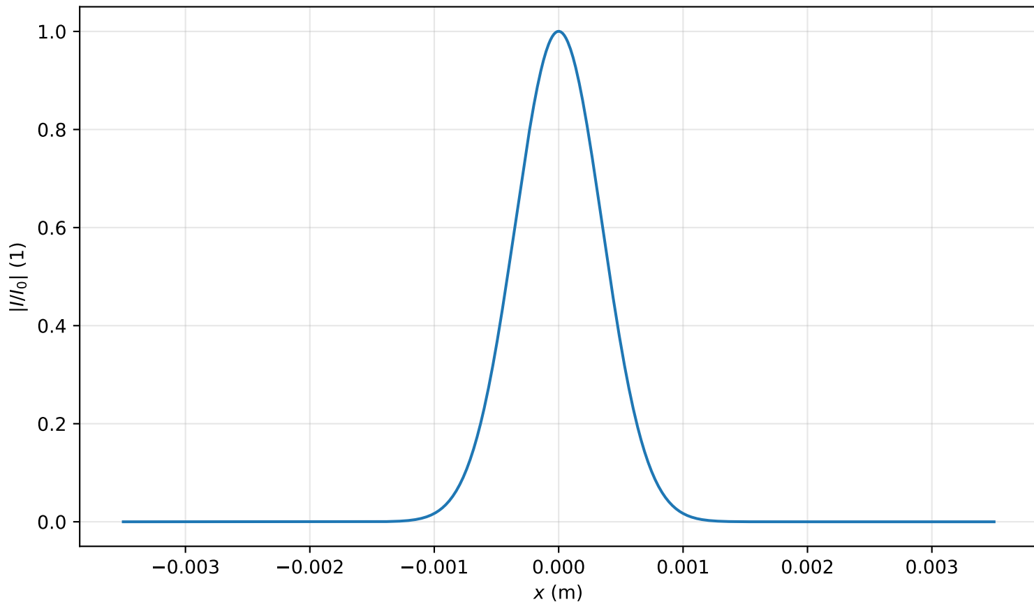
Intensity profile I(x, y = 0, z = 0.080m)/I_0 , P_{in}=0.3P_{cr} , artificial time
